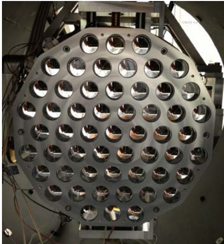
Figure 5 GRA inside the SCF-G facility
