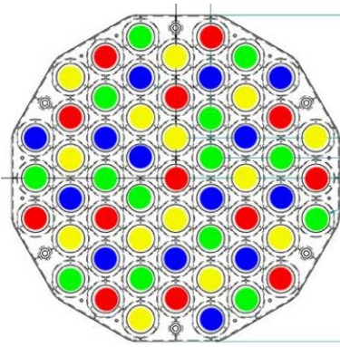
Figure 2 Azimuth rotation of CCRs on the GRA
