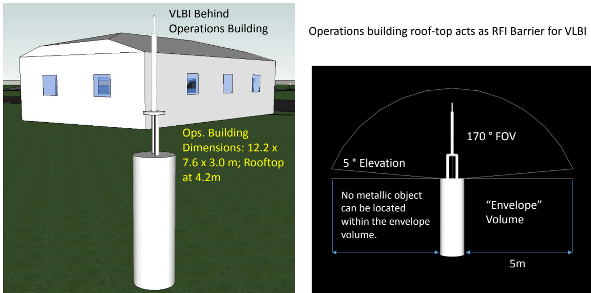
Figure 14: DORIS perspective near the operations building.
