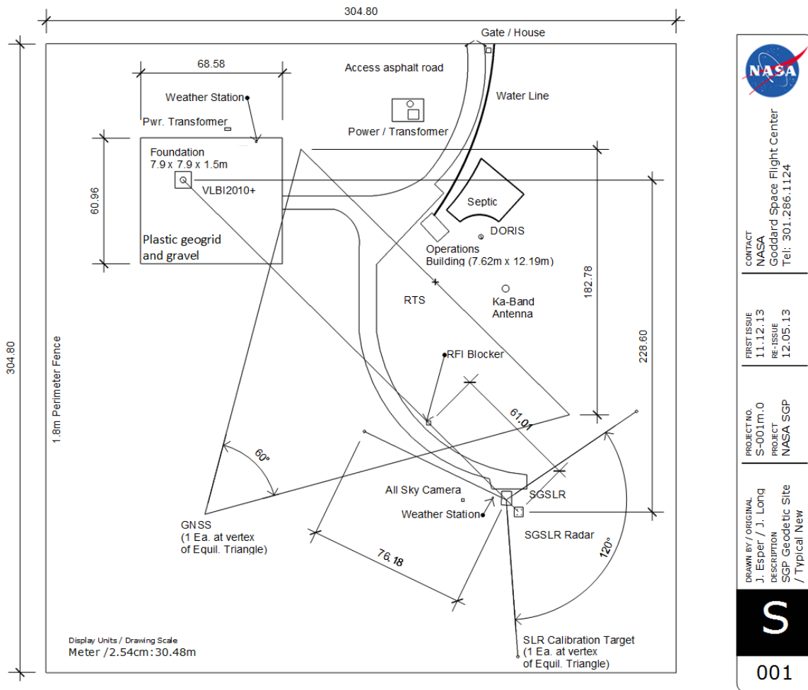
Figure 11: Typical NASA SGP site drawing with unencumbered terrain.
