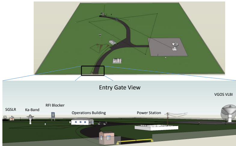
Figure 12: Idealized SGP CS layout and entry gate perspective (assumes flat terrain).
