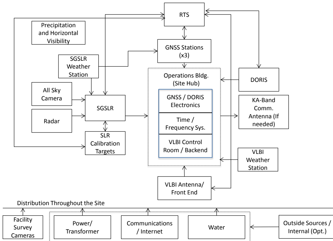
Figure 9: Typical NASA SGP Core Site Block Diagram
