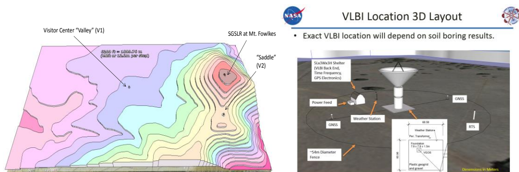
Figure 8: 3-D topographic model aids in selection of station configuration and site layout.
