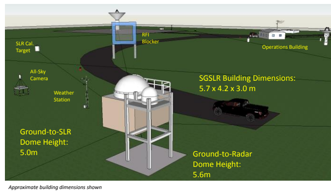
Figure 13: Perspective from SLR station, with RFIB in place.
